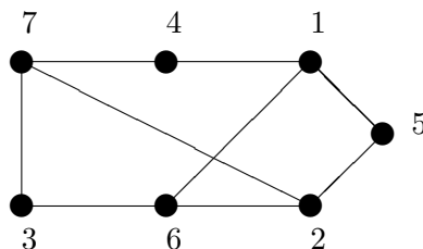
FIGURE 1. The Toeplitz graph T_7\langle 3, 4, 5 \rangle
