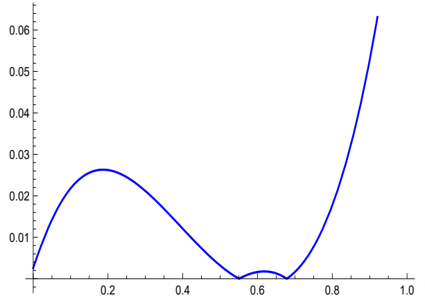
Figure 5: Graph of the absolute error of the approximate solution for \sigma(t) obtained by employing the proposed method in the presence of presice boundary data with \lambda_1 = 10^{-5} , discussed in Example 3.1.
