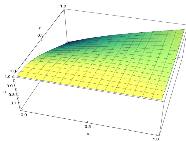
Figure 8: Approximate solution of u(x, t) , discussed in Example 3.1.1.
