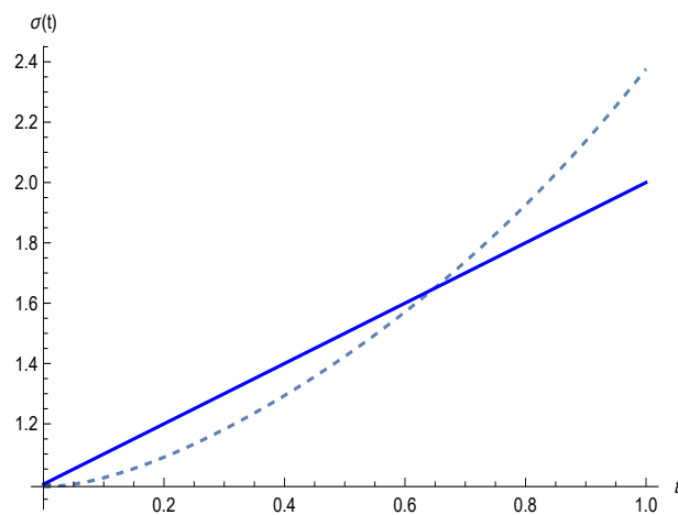
Figure 7: Graphs of the exact (thick line) and approximate (dashed line) solutions corresponding to the unknown function \sigma(t) , discussed in Example 3.1.1.
