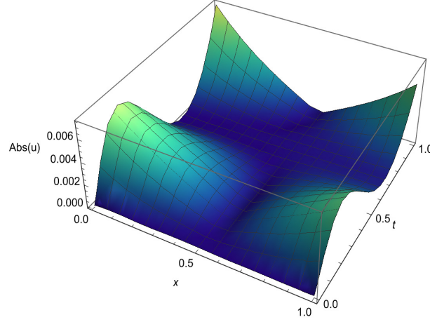
Figure 4: Graph of the absolute error of the approximate solution for u(x, t) obtained by employing the proposed method in the presence of presice boundary data with \lambda_1 = 10^{-5} , discussed in Example 3.1.
