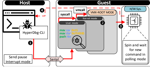
Figure 3: The overall view of the communication in HYPERDBG
