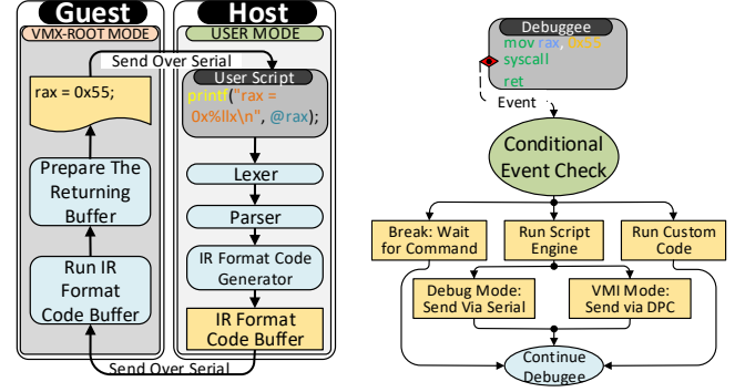
(a) HYPERDBGs script engine's (b) Script Engine invocation as an execution flow event
