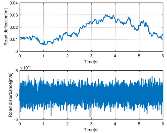
FIGURE 8 Road vertical displacement and velocity (Case 2) [Color figure can be viewed at wileyonlinelibrary.com ]
