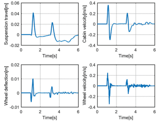
FIGURE 4 State response of active perturbed system (Case 1) [Color figure can be viewed at wileyonlinelibrary.com ]
