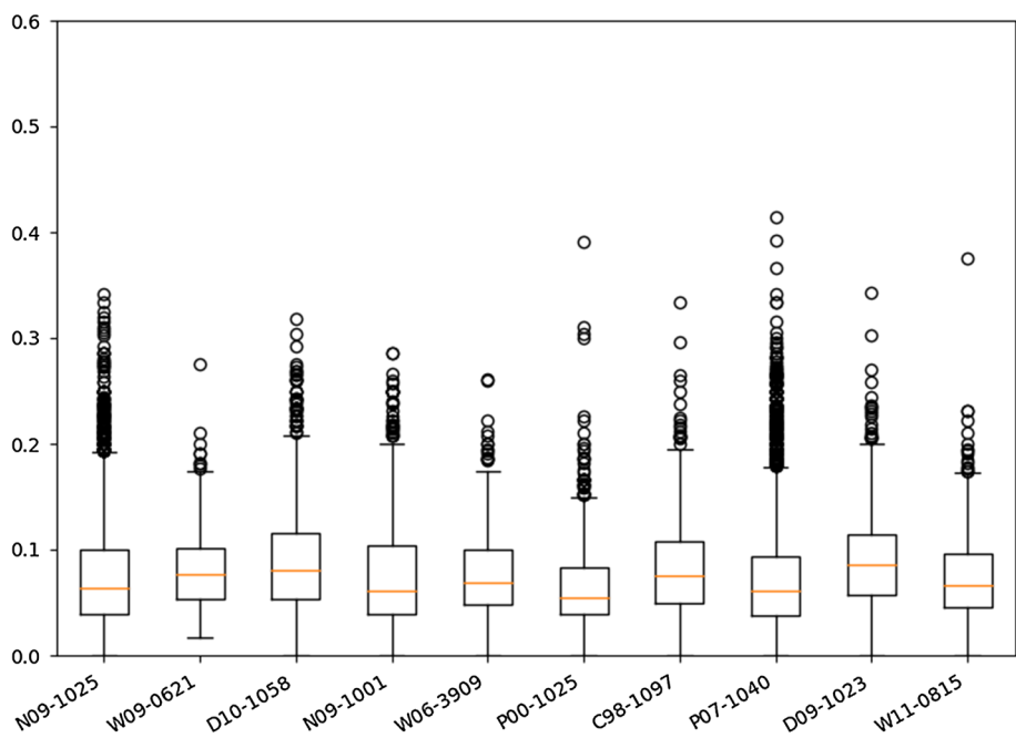
Fig. 8 JS values of unsolved-by-us citations with all reference sentences in test set reference documents
