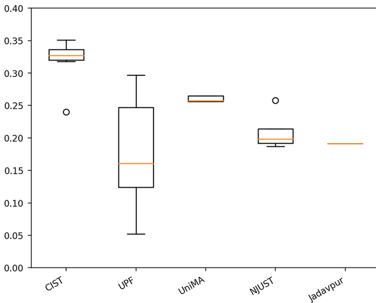
Fig. 3 Systems' performance on Task 2 (summaries vs. abstracts) with ROUGE-2 F_1 metric
