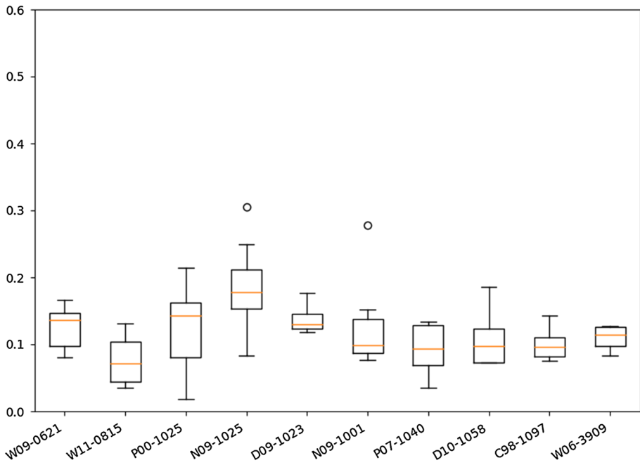
Fig. 12 JS values of unsolved-by-us citances with the reference span sentences (SR(c)s) in test set reference documents
