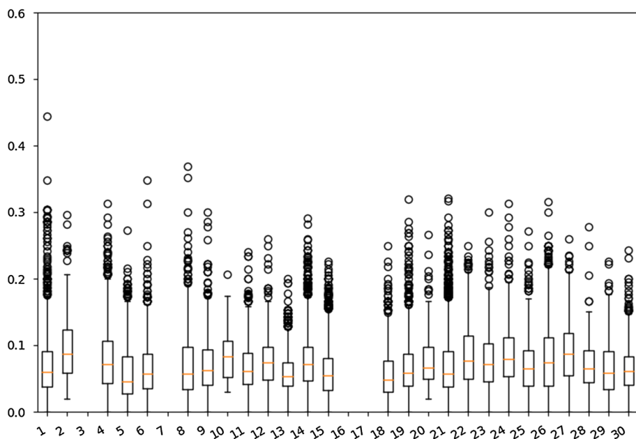
Fig. 6 JS values of unsolved-by-us citances with all the reference sentences in training set reference documents
