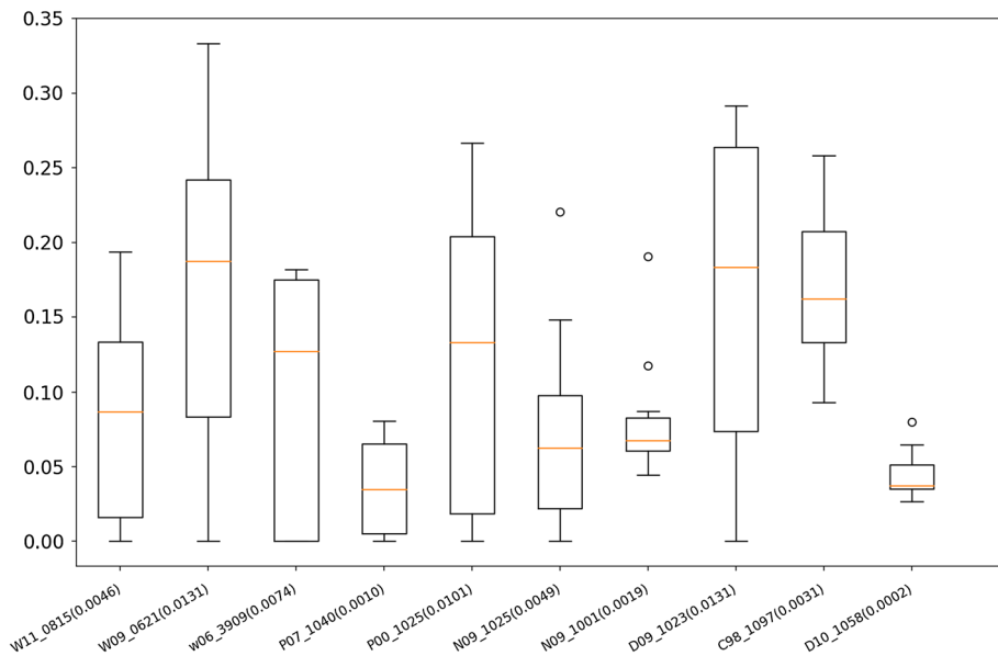
Fig. 4 Participating systems' best runs sentence overlap F_1 score for Task 1A by reference document. The variance is reported in parentheses
