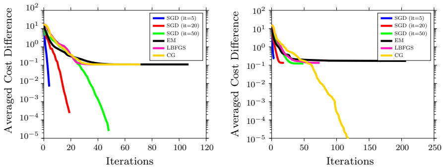
Fig. 8 Comparison of optimization methods on corel data ( d = 57 , n = 68,040 ). Y-axis: current objective values minus best objective. X-axis: number of function and gradient evaluations. Left: 7 number of components Right: 3 number of components
